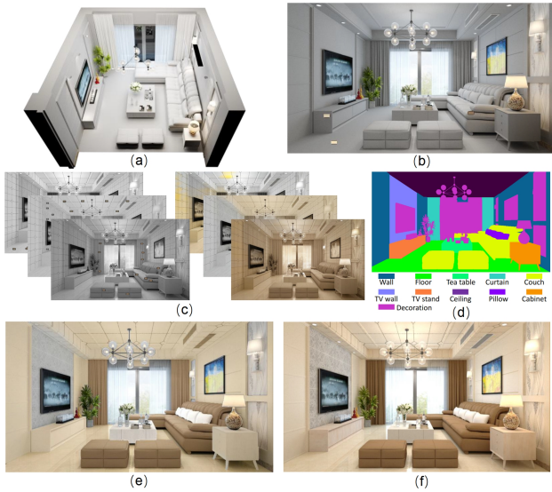
Figure 1: Given a 3D indoor scene (a) with a small set of user-specified colors (indicated by small color boxes) on its snapshot (b), our system suggests additional harmonious colors and allocates them to multiple layers of pre-rendered gray snapshots of the same scene under the same viewpoint for colorization (c). The colored multi-layer images are then merged together based on the semantic map (d) to generate a colored snapshot of the given scene respecting the user-designed color theme (e). Once a desired color theme is determined, the corresponding materials and colors can finally be attached to the given 3D scene for high-quality rendering (f).
