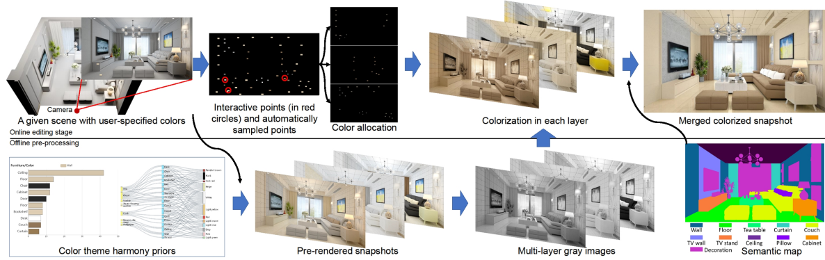
Figure 2: System overview. The offline pre-processing stage aims at generating multi-layer gray images for a given 3D indoor scene. In the online stage, our system suggests and samples more points based on a small set of user-specified colors, and chooses the proper layers for colorization. Finally, the colorized layers are merged to synthesize the final colored snapshot, with the help of the semantic map obtained in the offline stage.
